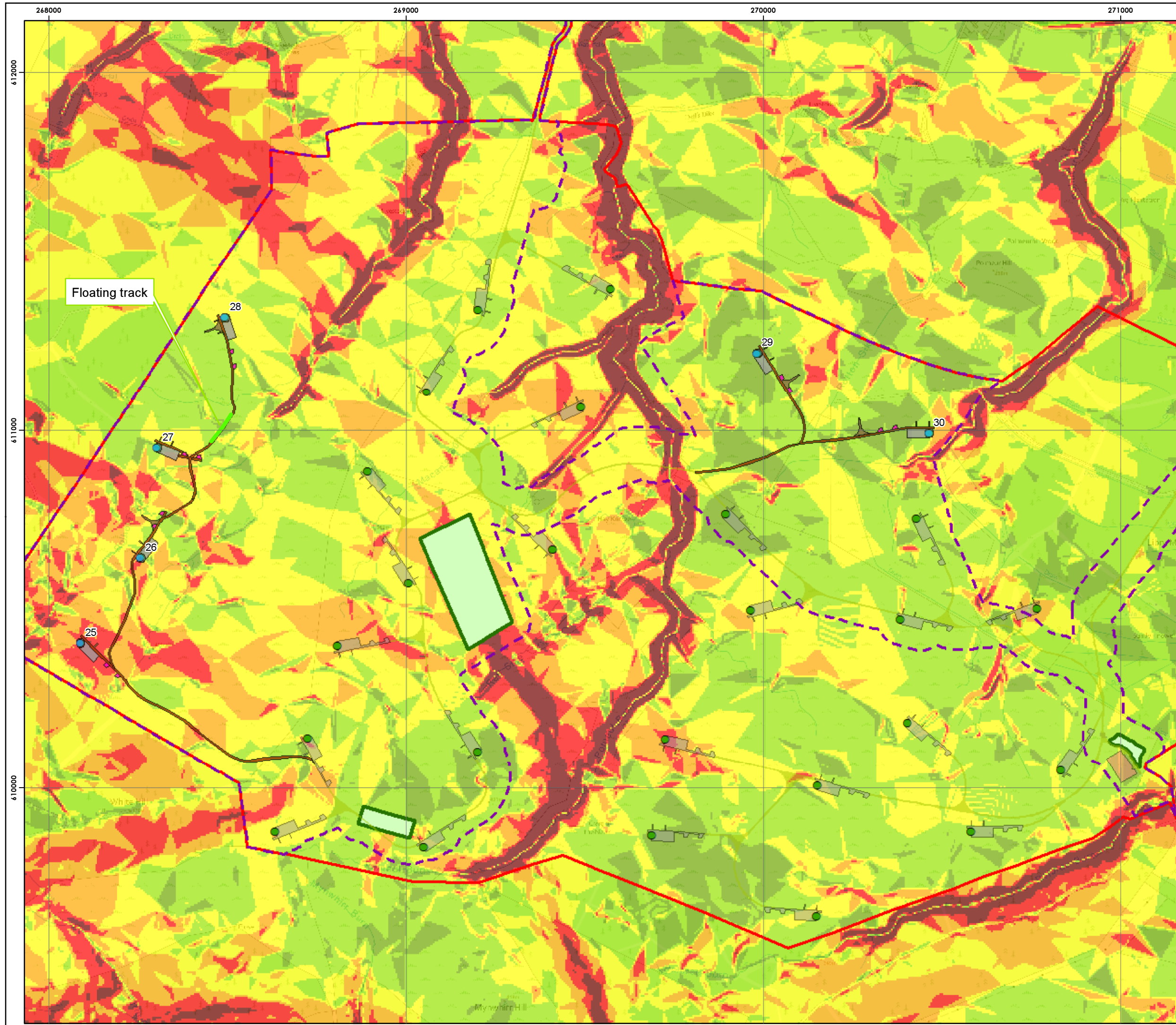
Figure 8.2.2 Slope Angle
