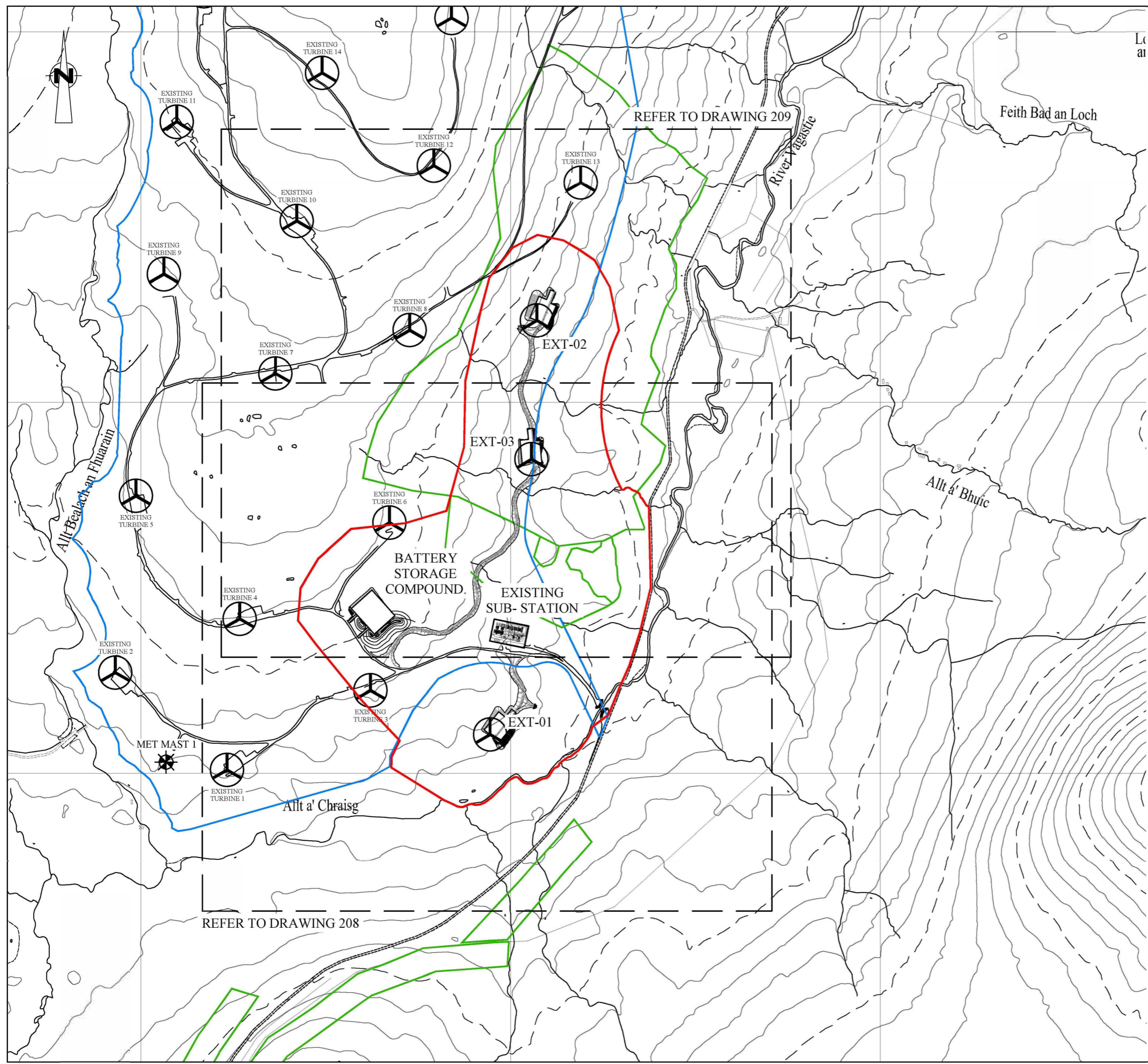
Figure 3.1a: Site Layout
